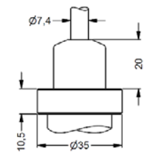
cable outlet, cable with ventilation tube (IP 68) 7
