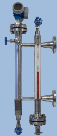
Magnetic Level Gauge-Dual Chamber
